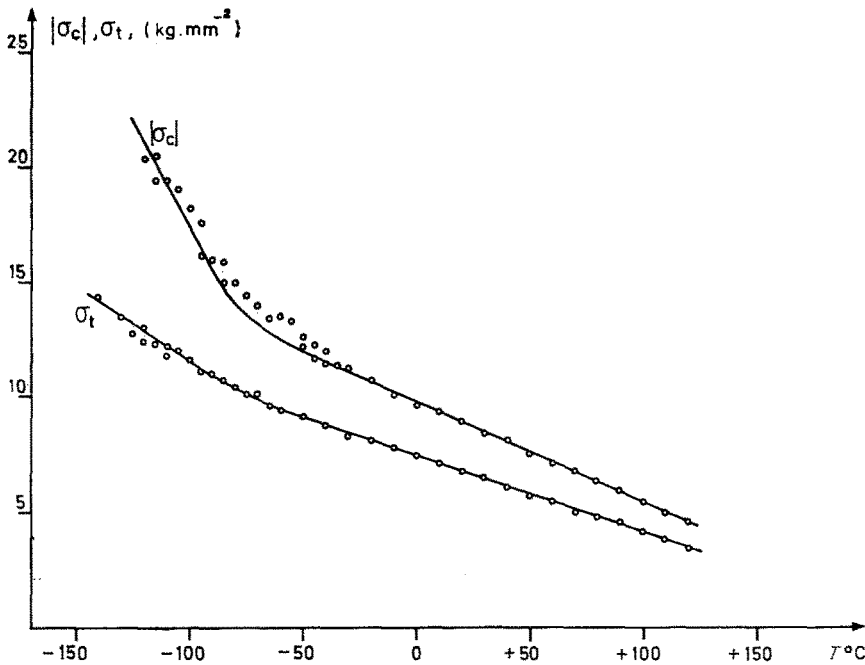
Figure 1 Plot of the engineering yield stress in uniaxial compression |\sigma_c| and in tensile tests \sigma_t versus temperature at a constant strain-rate \dot{\epsilon} = 4.16 \times 10^{-3} \text{ sec}^{-1} . The curves are generated from equations 1 and 2 using the constants given in table I.
